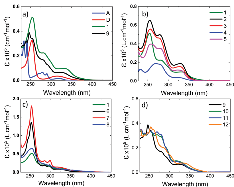
Fig. 4 Absorption spectra in dichloromethane. (a) Donor, acceptor and the unsubstituted D–A–D and D–A molecules, 1 and 9 ; (b) D–A–D molecules with the substituents on the donor, 1–5 ; (c) D–A–D molecules with the substituents on the acceptor 6 and 7 , and on both D and A units, molecule 8 ; (d) D–A molecules with substituents on the donor, 10–12 .
