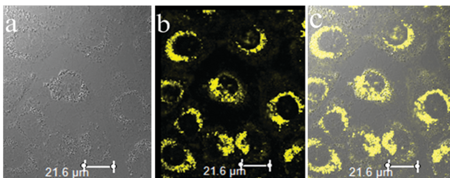
Fig. 15 Two-photon fluorescence images (at 800 nm) for A549 cells incubated with SPF-2 (50 \mu M) for 30 min. (a) Bright field; (b) fluorescence; and (c) overlay images of the A549 cells.
