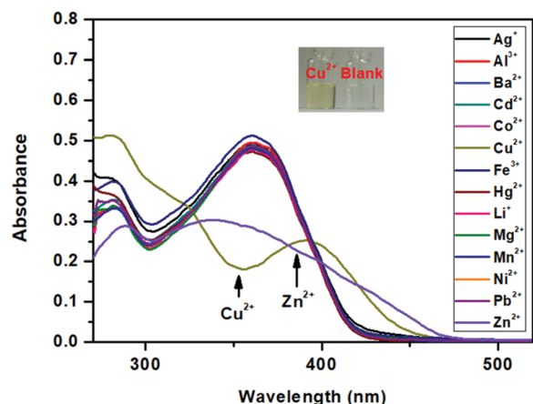
Fig. 10 The absorption spectra of SPF-1 (10 \mu M) upon addition of various metal ions (10 \mu M) in DMF/H 2 O (9:1, v/v).
