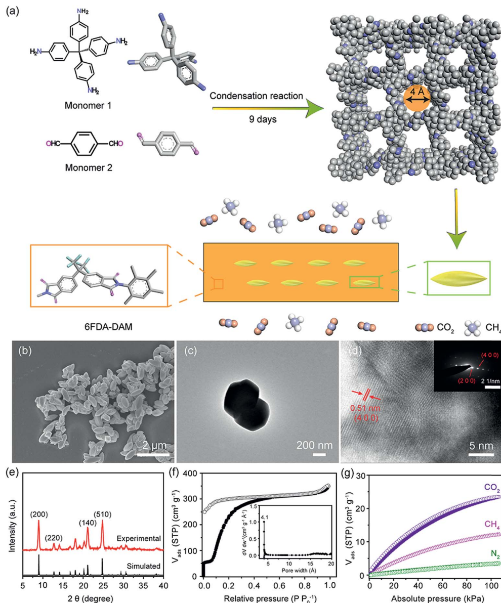
Fig. 1 (a) Schematic illustration of the preparation of COF-300 fillers and the fabrication of COF-300/6FDA-DAM MMMs for CO_2/CH_4 separation. (b) FESEM image of COF-300 crystals with a well-defined spindle shape. (c) TEM image of COF-300 crystals. (d) High resolution TEM image of COF-300 demonstrating an ordered lattice structure. The inset shows the SAED pattern of COF-300. (e) PXRD patterns of COF-300. The experimental pattern (top) matches well with the simulated pattern (bottom), indicating the successful preparation of high-quality COF-300 crystals. (f) N_2 sorption isotherm (77 K) of COF-300 crystals (adsorption: solid symbols; desorption: empty symbols). The inset shows the pore size distribution of COF-300 crystals calculated based on the slit mode using a Horvath-Kawazoe model. (g) CO_2 , CH_4 and N_2 sorption isotherms of COF-300 collected at 298 K (adsorption: solid symbols; desorption: empty symbols).
