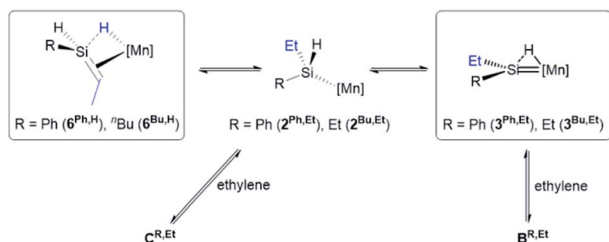
Scheme 7 Initial steps in the pathway proposed for reactions of silene hydride complexes [(dmpe)_2MnH(RHSi=CHMe)] ( 6^{Ph,H} ; R = Ph , 6^{Bu,H} ; R = n\text{-Bu} ) with ethylene to afford [(dmpe)_2MnH(RETSi=CHMe)] ( 6^{Ph,Et} ; R = Ph , 6^{Bu,Et} ; R = n\text{-Bu} ). [Mn] = Mn(dmpe)_2 . Intermediates B^{R,Et} and C^{R,Et} are analogous to intermediates B^R and C^R in Scheme 6, but with an ethyl group in place of one hydrogen atom on silicon. Only one isomer of 3 is shown. Boxes indicate complexes which have been isolated or spectroscopically observed.
