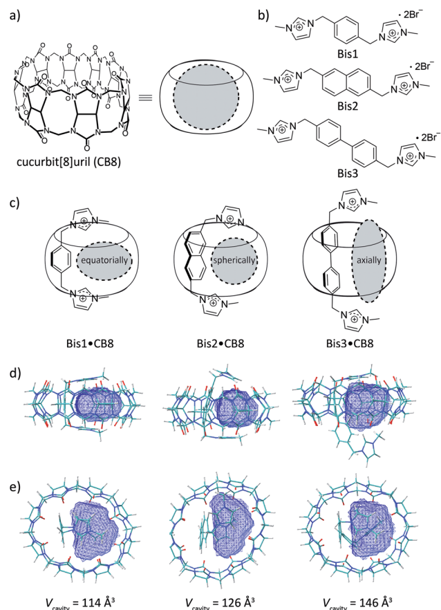
Fig. 1 Chemical structures of (a) CB8, (b) the bisimidazolium auxiliary guests, and (c) their schematic complexes with CB8; differently shaped cavities shown in grey. (d) and (e) show the side and top views of the DFT-optimized (wB97XD/3-21G* level of theory) binary complex structures with the respective accessible cavity volume ( V_{\text{cavity}} ) highlighted in blue.
