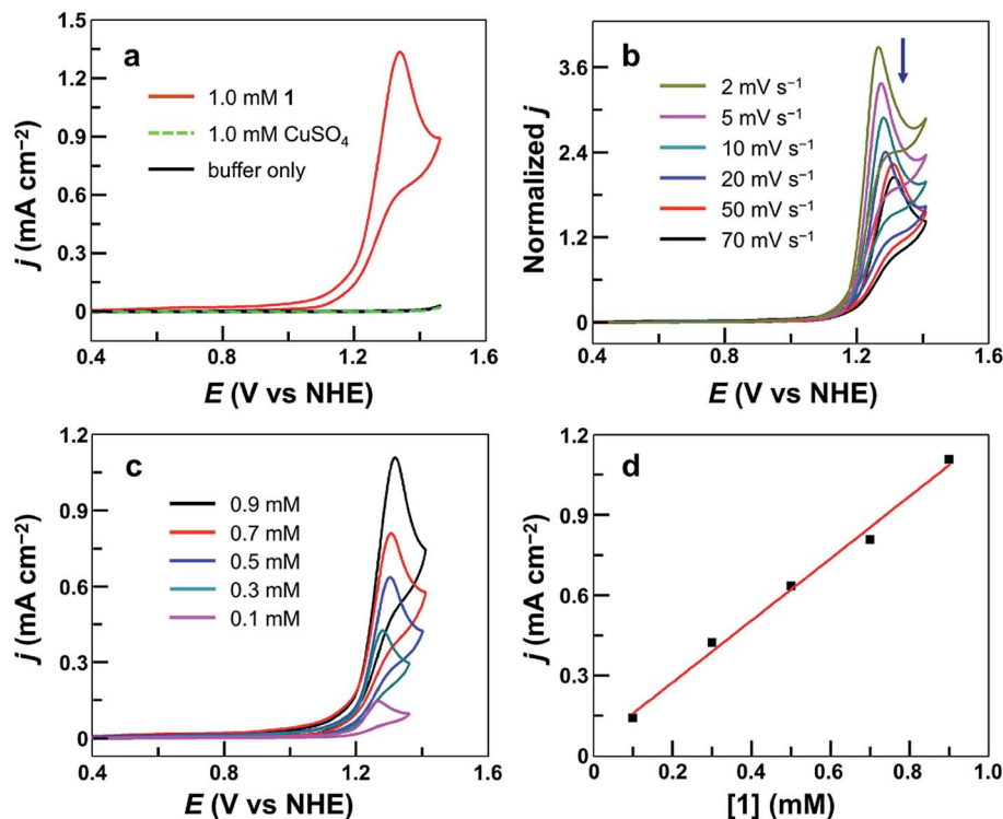
Fig. 2 (a) CVs of 1, CuSO 4 , and buffer-only solution at a 100 mV s -1 scan rate. (b) Normalized CVs of 0.50 mM 1 at different scan rates in mA cm -2 V -1/2 s 1/2 . (c) CVs of 1 at different concentrations. (d) Plot of catalytic peak current versus [1]. Conditions: FTO working electrode ( S = 0.25 cm 2 ), 0.10 M pH 7.0 phosphate buffer, and 20 °C.
