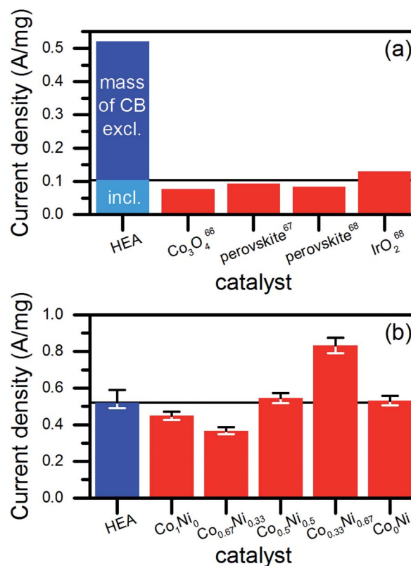
Fig. 7 Comparison of the mass-related current density or mass effectiveness of HEA NPs (water-based synthesis at low-power laser) to literature data (a) and to catalysts based on NPs from the laser ablation of Co x Ni 1-x targets, which were produced the exact same way as the HEA NPs. The black line in both diagrams marks the mass activity of the HEA catalyst for alkaline OER. The error bars in (b) represent the maximum deviation evaluated from three measurements in case of the HEA sample and the systematic error of the electrochemical measurement of 5% in case of the other samples.
