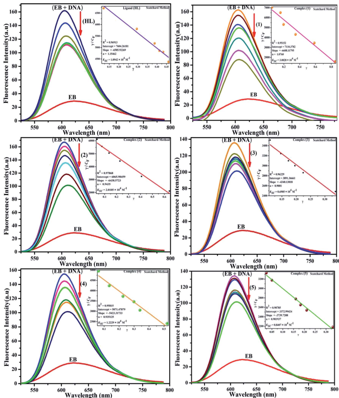
Fig. 5 Fluorescence quenching curve of EB-bound DNA in the presence of the ligand (HL) and its complexes (1–5). [DNA] = 100 \mu M, [complex] = 0–120 \mu M. Inset: Scatchard plot determining the association of the binding constant and the number of binding sites for the ligand (HL) and its complexes (1–5) to DNA.
