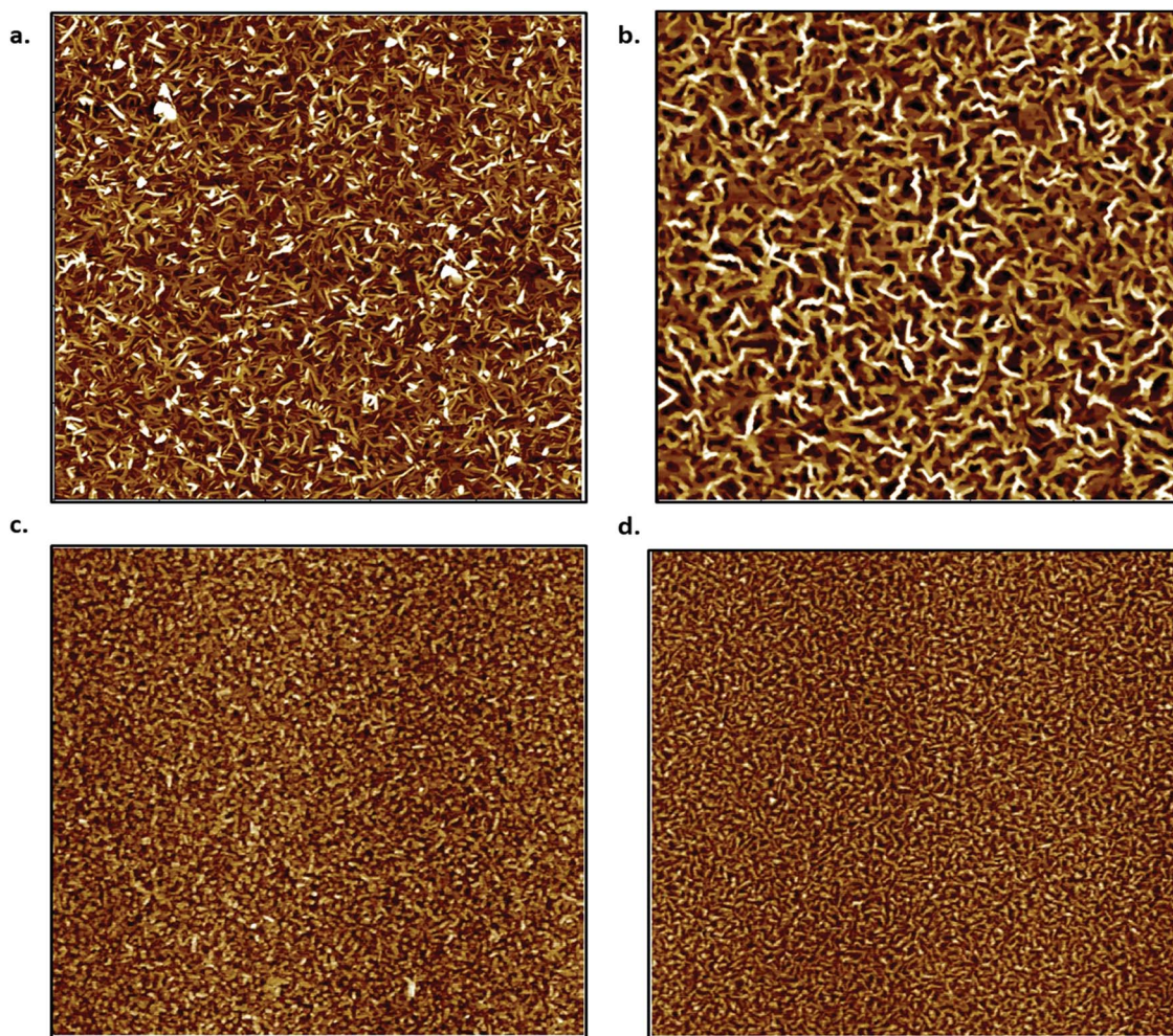
Fig. 5 AFM images of CuPc (a and c) and F 16 -CuPc (b and d) thin films deposited on SiO 2 substrates at 140 °C (a and b) and 20 °C (c and d). Images (a and b) are 5 \mu\text{m} \times 5 \mu\text{m} while (c and d) are 2.5 \mu\text{m} \times 2.5 \mu\text{m} .
