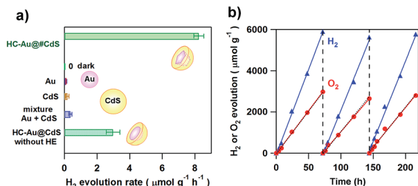
Fig. 5 (a) The comparison of the \text{H}_2 evolution rate for HC-Au( d_{\text{Au}} = 5.5 \text{ nm} )@#CdS( l_{\text{CdS}} = 1.9 \text{ nm} ), Au colloid, CdS, and a mixture of Au and CdS under red-light illumination ( \lambda_{\text{ex}} = 640 \text{ nm} ) or dark conditions. (b) Repeated water splitting by HC-Au( d_{\text{Au}} = 12.1 \text{ nm} )@#CdS( l_{\text{CdS}} = 2.1 \text{ nm} ) under red-light illumination. Figures are taken from ref. 59.
