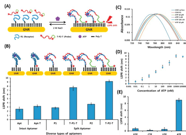
Fig. 10 (A) Schematic representation of the developed LSPR apta-sensor for ATP detection based on structure assembly inducing LSPR shift using split-aptamers labelled with TAMRA dye and a random sequence tail. (B) Optimisation of truncation of the aptamer and introduction of TAMRA into the aptamer to achieve maximum LSPR. (C) Shift in LSPR in response to various concentrations of ATP from 10 pM to 10 \mu M. (D) Linear fitting of the LSPR signals for ATP concentrations. (E) Specificity analysis of the developed LSPR based apta-sensor for relevant nucleotides. Adapted with permission from ref. 103. Copyright (2015) Elsevier.
