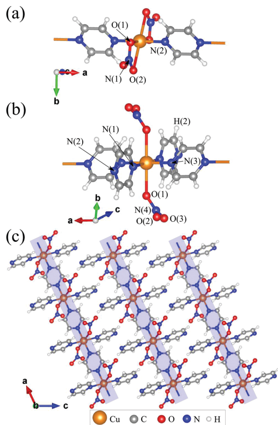
Fig. 1 Local environments of the Cu 2+ ions in (a) 1 and (b) 2 . (c) Structure of 2 demonstrating the packing of chains.
