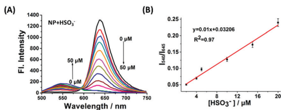
Fig. 1 (A) The fluorescence responses of 10 \mu\text{M} NP upon addition of \text{NaHSO}_3 (0–50 \mu\text{M} ). \lambda_{\text{ex}} = 446 \text{ nm} . (B) The relationship between fluorescence ratio ( I_{540}/I_{645} ) and [\text{HSO}_3^-] .
