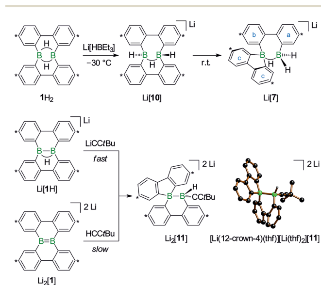
Scheme 6 Reaction of 1H_2 with Li[HBet_3] at -30^\circ C to give Li[10], which isomerizes to Li[7] at room temperature (top). Compound Li_2[11] forms in both reactions, tBuCClLi/Li[1H] and tBuCCH/Li_2[1] (bottom; carbon atoms marked with asterisks bear tBu substituents). Molecular structure of [Li(12-crown-4)(thf)][Li(thf)_2][11] in the solid state. The solvent-separated cations, phenyl-bonded tBu groups, and all CH atoms are omitted for clarity.
