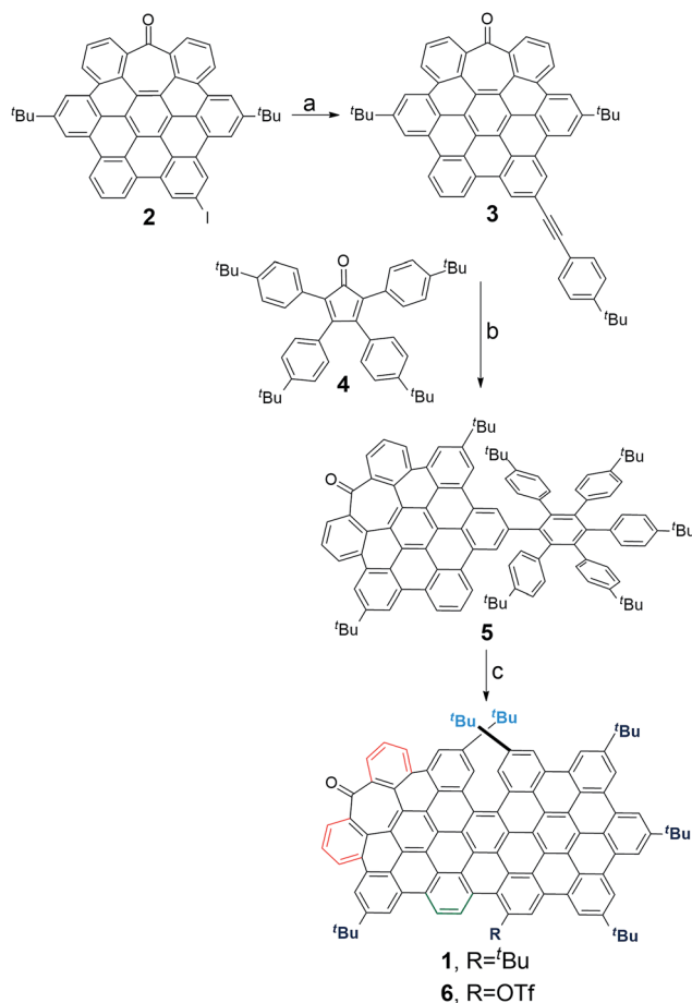
Scheme 1 Synthesis of compound 1 . Reagents and conditions: (a) 4-tert-butylphenylacetylene, PdCl 2 (PPh 3 ) 2 , CuI, NEt 3 , THF, RT, 16 h, 99%; (b) Ph 2 O, reflux, 8 h, 34%; (c) DDQ, CF 3 SO 3 H, CH 2 Cl 2 , 0 °C, 10 min, 1 (46%) and 6 (5%).
