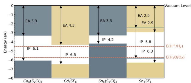
Fig. 6 Electron affinities (EA) and ionisation potentials (IP) for the candidate materials, from DFT calculations of non-polar crystal terminations. The water redox potentials (dashed orange lines) are also shown. For Sn 4 SF 6 , a dipole correction was added resulting in lower and upper (blue solid lines) bounds for the IP and EA values.
