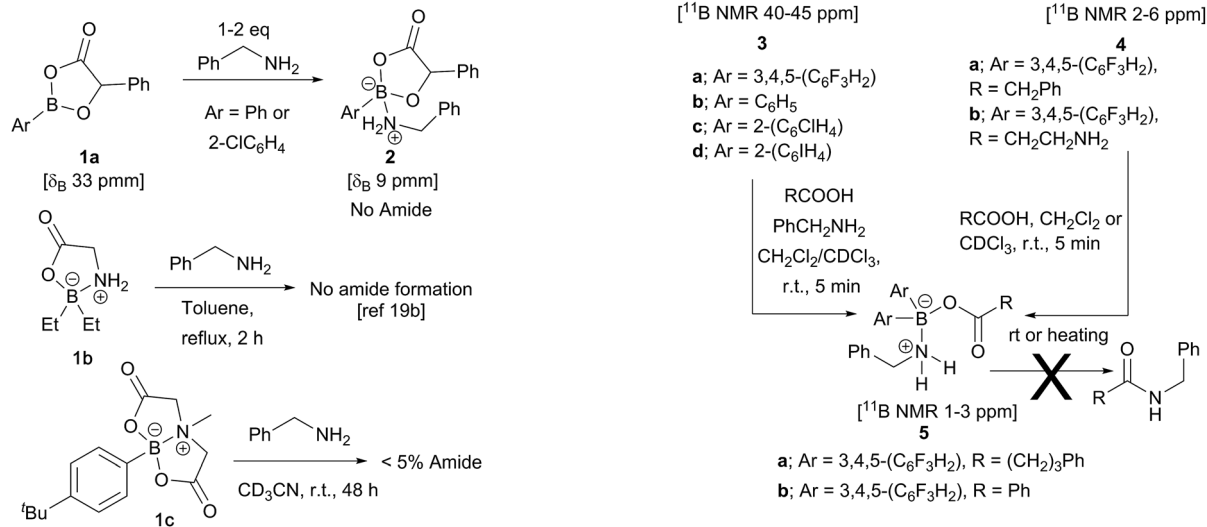
Scheme 3 Monomeric acyloxyboron species typically show low reactivity towards amines.
