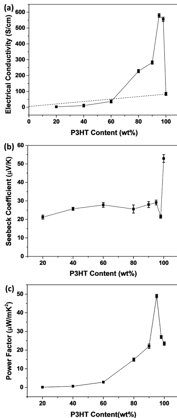
Fig. 9 (a) Electrical conductivity, (b) Seebeck coefficient and (c) power factor of P3HT/CNT ( d < 8 nm) composite films with P3HT content (wt%) of 20 wt%, 40 wt%, 60 wt%, 80 wt%, 90 wt%, 95 wt%, 98 wt% and 100 wt%. The dashed line is the estimated electrical conductivity based on the parallel connected mixture model.
