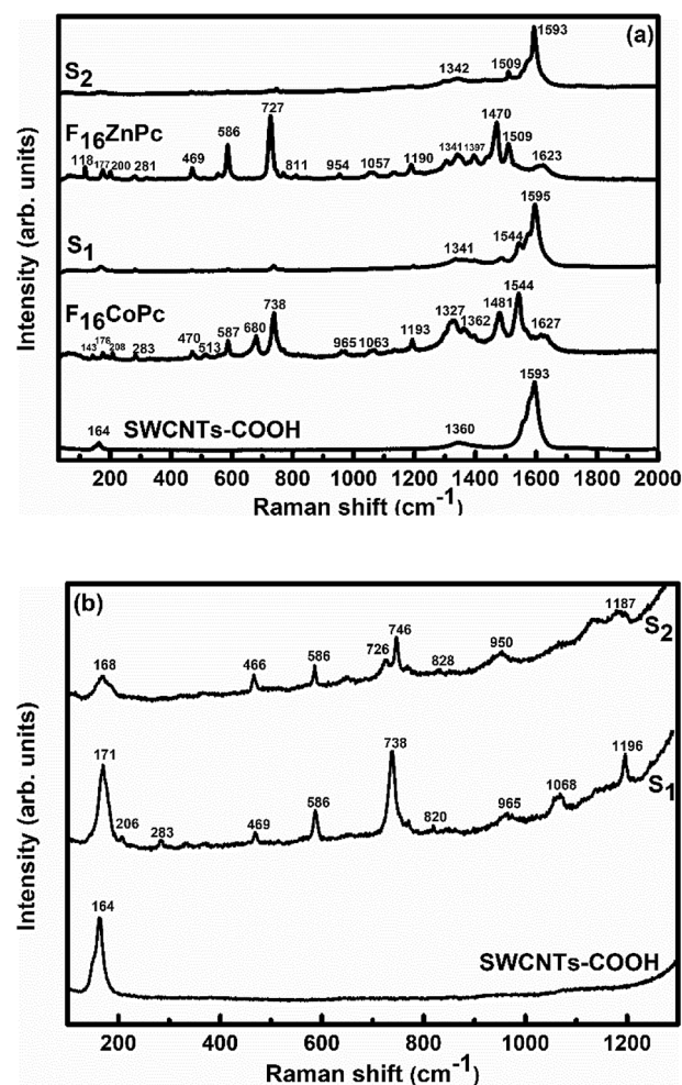
Fig. 3 Raman spectra of (a) \text{SWCNTs-COOH} , \text{F}_{16}\text{CoPc} , S_1 , \text{F}_{16}\text{ZnPc} and S_2 hybrids, and (b) \text{SWCNTs-COOH} , S_1 and S_2 hybrids in the 30– 1300\text{ cm}^{-1} range (magnified view).
