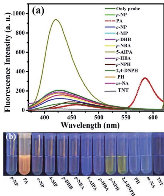
Fig. 4 (a) Fluorescence spectra of L (20 \mu M) in the absence and presence of 200 \mu M various aromatic compounds ( \lambda_{\text{ex}} = 314 nm, slits: 2.5 nm/5 nm; slits: 1.0 nm/5 nm for 5-AIPA); (b) photograph of probe solutions with different aromatic compounds under 365 nm UV lamp.
