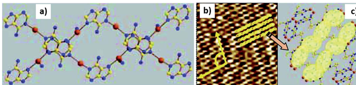
Fig. 24 (a) Double-stranded coordination helicate 2. (b) AFM image of 2 on HOPG surface. Image size is 400 \times 400 \text{ Å}^2 ; (c) proposed model of adenine-silver helicate deposition. (Reproduced with permission from ref. 118 © 2007 American Chemical Society).
