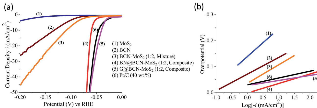
Fig. 21 HER electrocatalytic performance comparison. (a and b) Linear sweep voltammogram polarization curves and Tafel plots of (1) MoS 2 , (2) BCN, (3) BCN-MoS 2 (1 : 2, mixture), (4) BN/BCN-MoS 2 (1 : 2, composite) (5) G/BCN-MoS 2 (1 : 2, composite) samples including (6) Pt/C (40 wt%).
