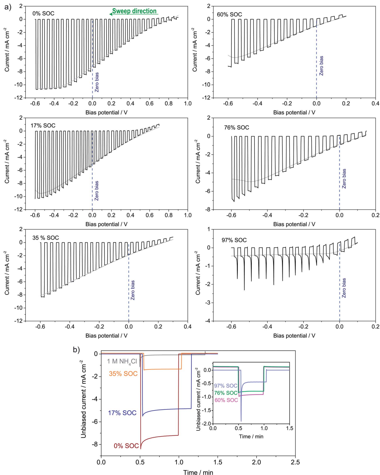
Fig. 6 (a) LSVs on pn + Si/TiO 2 recorded in the solar flow battery cell using the same concentration anolyte and catholyte as in the battery cycling tests. The electrolytes were brought to the indicated SOC in the RFB cell. (b) The unbiased photocurrent density at the same SOC recorded as the light is turned on (at the time ca. 0.5 minute); the inset shows the higher SOC.
