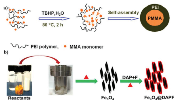
Fig. 1 (a) Synthesis of PMMA/PEI core-shell nanoparticles. Reproduced with permission from ref. 37. Copyright 2011 Elsevier. (b) Schematic illustration of the Synthesis of Fe_3O_4@DAPF ferromagnetic nanorods. Reproduced with permission from ref. 38. Copyright 2015 American Chemical Society.
