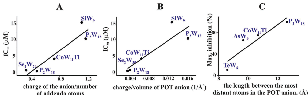
Fig. 7 Structure–activity correlations of different POTs for ATPases inhibition. (A) Correlation between the \text{IC}_{50} values of five POTs ( \text{IC}_{50} lower than 16\ \mu\text{M} ) of \text{Ca}^{2+} -ATPase inhibition and their charge density expressed as charge of the POT divided by its number of W atoms. (B) Correlation between the \text{IC}_{50} values of five POTs ( \text{IC}_{50} lower than 16\ \mu\text{M} ) against \text{Ca}^{2+} -ATPase and the charge density expressed as charge of the POT divided by its volume (in \text{\AA}^{-3} ). (C) Correlation between the percentage of maximum inhibition of four POTs (applied with the same concentration of 10\ \mu\text{M} ) against \text{Na}^+/\text{K}^+ -ATPase and POT size expressed as the length between the most distant atoms in the POT anion (in \text{\AA} ).
