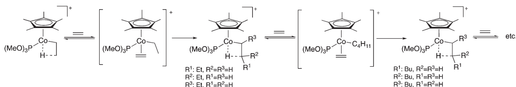
Scheme 3 Mechanism of the polymerization of ethylene. Adapted with permission from ref. 24. Copyright of the American Chemical Society (1990).
