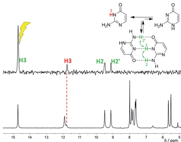
Fig. 3 1 H NMR spectrum (bottom) and differential 1 H NOE spectrum (top, irradiation at 14.7 ppm) of isocytosine in DME/DMF- d 7 solution at -120 °C confirming the dimer formation. The signal indicated by a red dashed line is the exchange signal of H3 in the isocytosine monomer.
