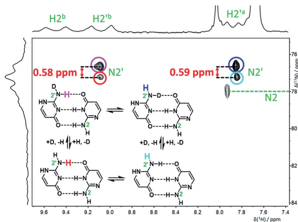
Fig. 4 H,N-HSQC spectrum of 15 N- and partially 2 H-labelled isocytosine in DME/DMF- d 7 at -120 °C, showing the deuterium-induced isotopic shifts of nitrogen N2' caused by isotope exchange of the hydrogen atoms involved and not involved in intermolecular hydrogen bonding (H2 b and H2' a , respectively).
