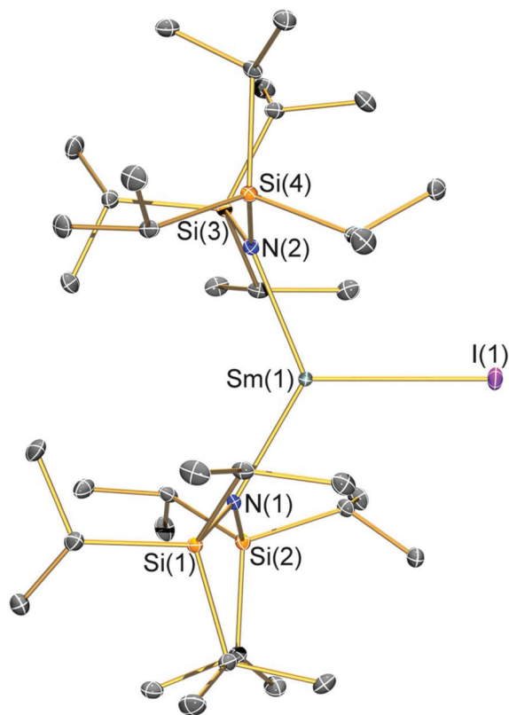
Fig. 4 Molecular structure of [\text{Sm}(\text{N}^{\text{H}})(\text{I})] ( 2-I ) with selective atom labelling. Displacement ellipsoids set at a 30% probability level and hydrogen atoms are omitted for clarity. Selected bond lengths [Å]: \text{Sm}(1)-\text{I}(1) 3.0199(7), \text{Sm}(1)-\text{N}(1) 2.323(3), and \text{Sm}(1)-\text{N}(2) 2.289(3). Selected bond angles [°]: \text{N}(1)-\text{Sm}(1)-\text{N}(2) 128.07(10), \text{N}(1)-\text{Sm}(1)-\text{I}(1) 119.75(7), and \text{N}(2)-\text{Sm}(1)-\text{I}(1) 112.16(7).
