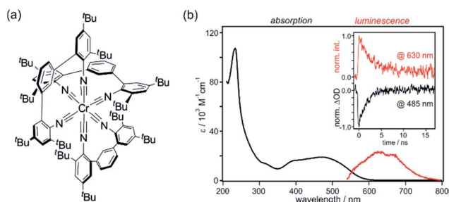
Fig. 10 (a) Chemical structure of the \text{Cr}(\text{CN}^{\text{tBu}}\text{Ar}_3\text{NC})_3 complex. 19 (b) UV-Vis absorption and luminescence spectra of \text{Cr}(\text{CN}^{\text{tBu}}\text{Ar}_3\text{NC})_3 in de-aerated THF at 20 °C. Excitation occurred at 450 nm. Inset: luminescence decay at 630 nm (red) and absorption bleach recovery at 485 nm (black) following excitation at 532 nm with pulses of \sim 30 ps duration. Adapted with permission from ref. 19. Copyright 2017 American Chemical Society.
