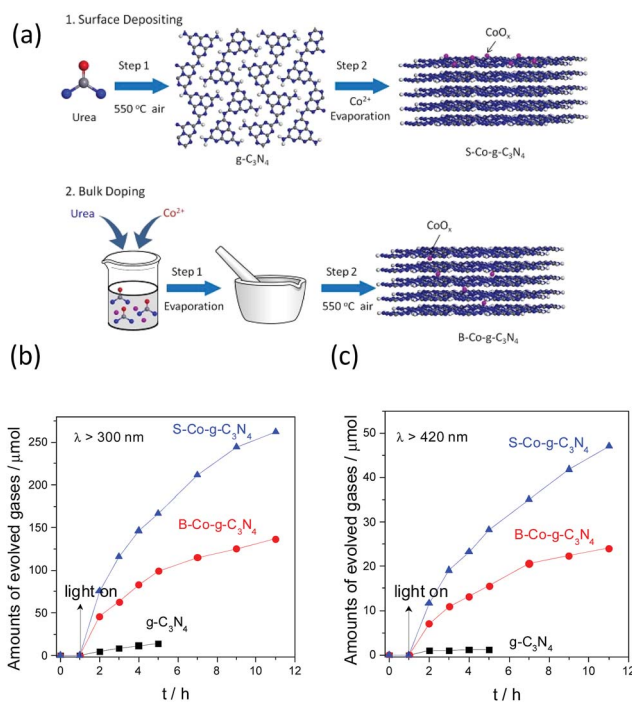
Fig. 11 (a) Schematic illustration of surface deposition and bulk doping modification of \text{g-C}_3\text{N}_4 . Photocatalytic water oxidation activities of the \text{g-C}_3\text{N}_4 , \text{B-Co-g-C}_3\text{N}_4 and \text{S-Co-g-C}_3\text{N}_4 samples under (b) UV ( \lambda > 300 \text{ nm} ) and (c) visible light ( \lambda > 420 \text{ nm} ) irradiation. Reprinted with permission from ref. 107. Copyright 2016, American Chemical Society.
