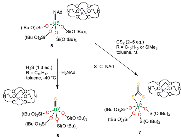
Scheme 3 Syntheses of the terminal U V trithiocarbonate complex, [K(2.2.2-cryptand)][U(CS 3 ){OSi(OtBu) 3 ] 4 ] ( 7 ), and the terminal U V sulfide complex, [K(2.2.2-cryptand)][US(OSi(OtBu) 3 ] 4 ] ( 8 ).
