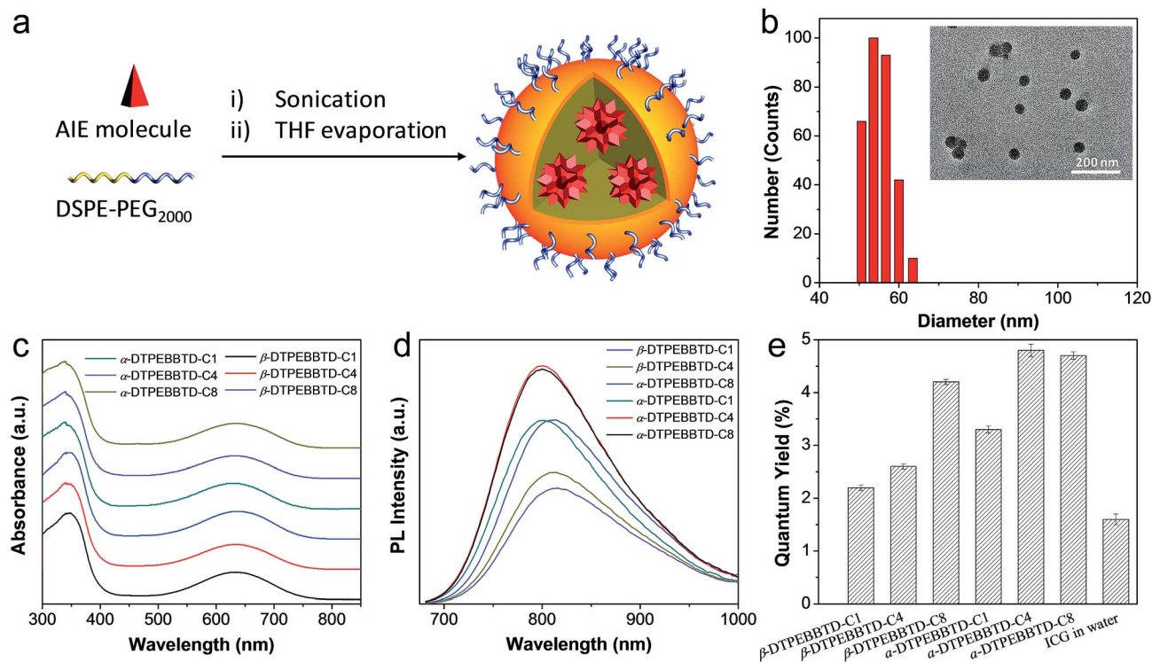
Fig. 2 Preparation and characterization of the AIE NPs. (a) Schematic illustration of AIE NP preparation. (b) Representative LLS and TEM results of α-DTPEBBTD-C4 based AIE NPs. (c) UV-vis absorption and (d) PL spectra of the AIE NPs in water. (e) Quantum yields of the AIE NPs and ICG in water.
