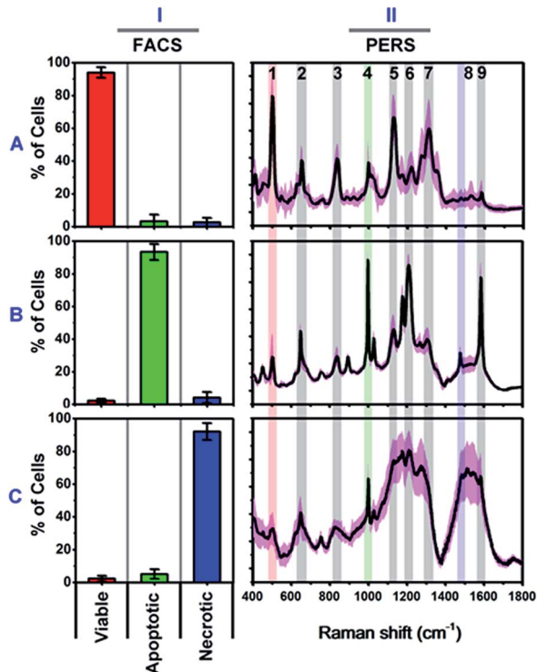
Fig. 2 Characterized flow cytometry (FACS) (I) and plasmonic-enhanced Raman spectra (PERS) (II) of reference viable (A), apoptotic (B) and necrotic cells (C). The black lines in the PERS spectra show the averaged spectra from 30 trials of measurements, and the pink colour indicates their standard deviation ( n = 30 ). The red (1), green (4) and blue (8) colour in the PERS spectra indicates the most representative bands in each population.
