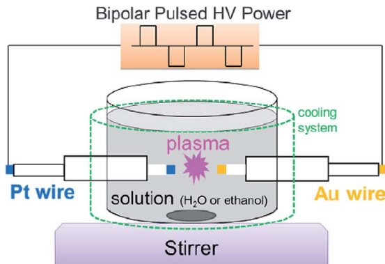
Fig. 14 Image of a synthesis apparatus of a gold/platinum alloy by in-liquid plasma using gold and platinum electrodes. Reproduced from Hua and coworkers. 157 Copyright 2013 by Elsevier.
