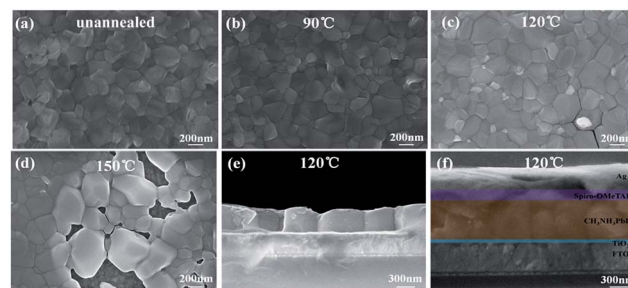
Fig. 2 SEM images of the perovskite films deposited via LFCVD procedure on FTO/c- \text{TiO}_2 , (a) before and after annealing at (b) 90\text{ }^\circ\text{C} , (c) 120\text{ }^\circ\text{C} and (d) 150\text{ }^\circ\text{C} for 30 min, respectively. The cross-section SEM image of (e) the perovskite film after annealing at 120\text{ }^\circ\text{C} for 30 min, (f) the multilayer structure in a complete photovoltaic structure.
