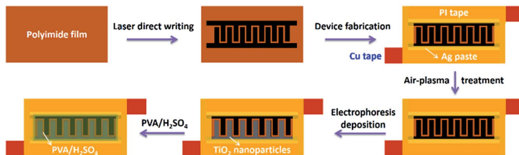
Fig. 1 Schematic illustration for the fabrication of a carbon/ \text{TiO}_2 micro-supercapacitor with photo-rechargeable capability.
