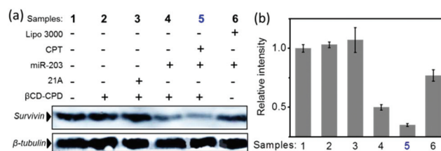
Fig. 6 (a) WB analysis of inhibition of endogenous survivin protein expression in HeLa cells treated with different complexes (10 \mu M) or transfection of naked miR-203 with Lipo 3000; (b) intensity of endogenous survivin protein expression in the WB analyzed with ImageJ software. Error bar was calculated from three independent experiments.
