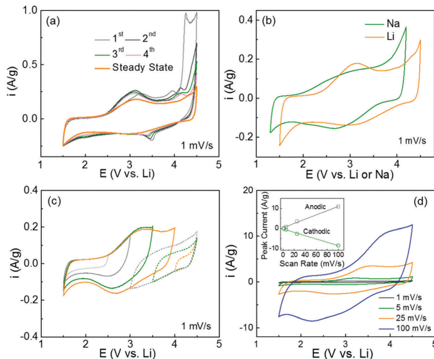
Fig. 5 Cyclic voltammetry (CV) measurement of the hybrid electrode (PDA-2, 39 wt%) in Li- and Na-cells. (a) The first four and steady-state CV scans at 1 mV s -1 in a Li-cell. (b) Comparison of steady-state CV scans in Li- and Na-cells. (c) Potential-dependent and (d) rate-dependent CV scans in Li-cells. Peak current of the electrode as a function of scan rate is shown in the inset of (d). The voltage window of the CV scans in the Li-cells was 1.5–4.5 V vs. Li in 1 M LiPF 6 in a mixture of ethylene carbonate (EC) and dimethyl carbonate (DMC) (3 : 7 volume ratio) and the voltage window in Na-cells was 1.3–4.2 V vs. Na in 1 M NaPF 6 in a mixture of EC and DMC (3 : 7 volume ratio).
