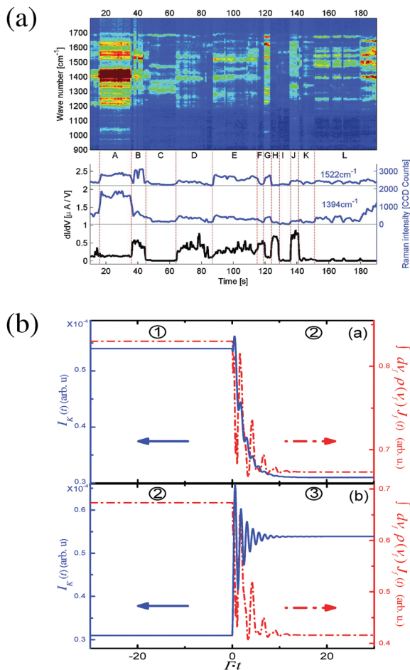
Fig. 7 Time-dependent fluctuations in simultaneously measured electro- nical conductance and Raman response in molecular junctions. Shown are (a) experimental data and (b) a theoretical analysis. (a) Reprinted with permission from D. R. Ward, N. J. Halas, J. W. Ciszek, J. M. Tour, Y. Wu, P. Nordlander and D. Natelson, Nano Lett. , 2008, 8 , 919–924. Copyright (2008) American Chemical Society. (b) Reprinted with permission from [T.-H. Park and M. Galperin, Phys. Rev. B: Condens. Matter Mater. Phys. , 2011, 84 , 075447.] Copyright (2011) by the American Physical Society. http://dx.doi.org/10.1103/PhysRevB.84.075447 .
