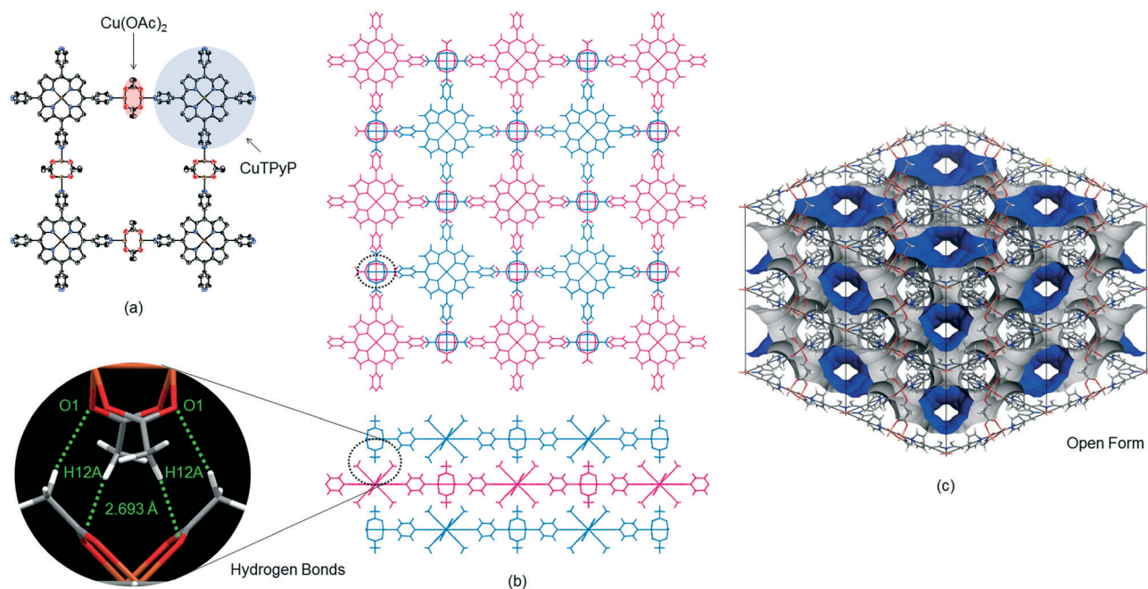
Fig. 1 (a) The 2.2 nm square grid of 1. Color scheme: C = gray; N = blue; O = red; Cu = brown. For clarity, the solvent molecules are not shown. (b) The stacking of 2D sheets in 1, with blue and red representing adjacent layers. (c) The crystal packing of 1 in the open form. For clarity, guest molecules and H atoms have been omitted.
