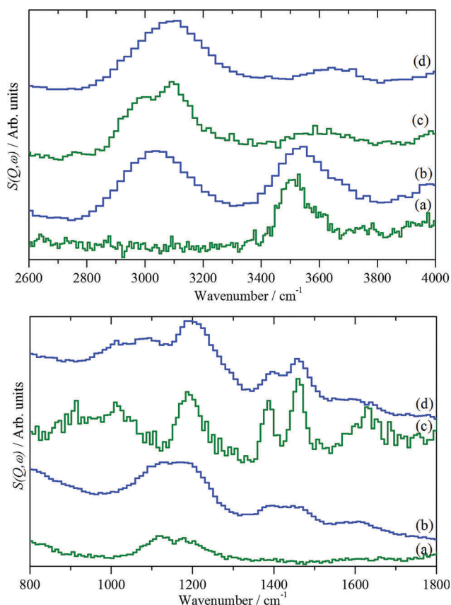
Fig. 15 INS spectra of H-ZSM5 under different conditions for the MTH reaction. 74 (a) The clean catalyst after dehydration at 350 °C and reaction with methanol at: (b) 350 °C for 1 hour, (c) 350 °C for 3 days and (d) 400 °C for 3 days. Upper part: the C–H and O–H stretch region. Lower part: the fingerprint region.
