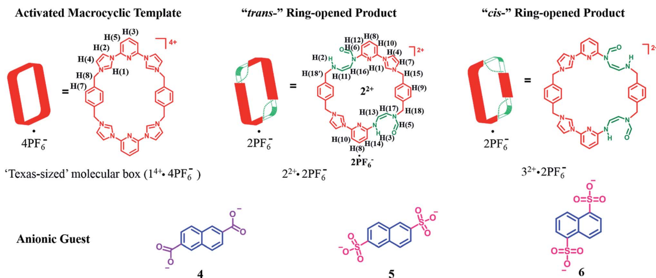
Scheme 1 Structures of the "Texas-sized" molecular box ( 1^{4+} \cdot 4PF_6^- ) and its " trans -" and " cis -" imidazolium ring-opened products. Also shown are the dianionic guest molecules used in this study.
