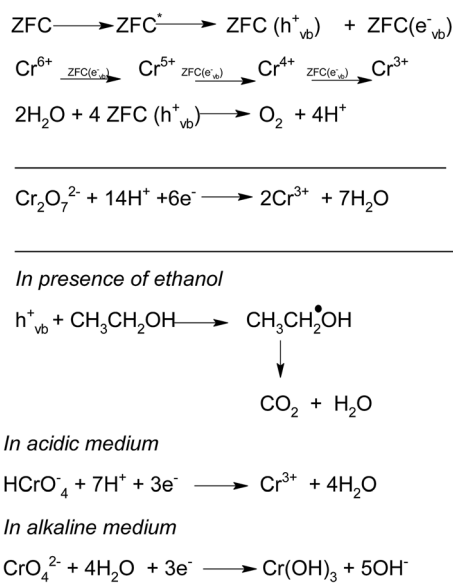
Scheme 1
