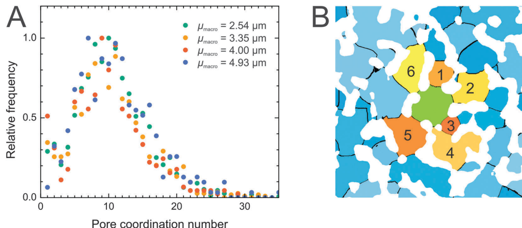
Fig. 5 (A) Distribution of pore coordination numbers as derived by MISA. The four silica monoliths share highly similar distributions with close to 75% of pores surrounded by 5–15 neighbors; 5–8% of pores have \geq 20 neighbors. (B) 2D view (slice) of a compartmentalized macropore space (white – silica skeleton, black – pore throats, color – pores). The central pore (green) in the image shares throat pixels with six neighbors (yellow to tangerine). Pores that do not share throat pixels with the central pore are colored in shades of blue. In the 3D reconstruction, the central pore is coordinated by ten neighbors.
