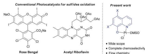
Fig. 1 Visible light photocatalysts for the photooxidation of sulfides.
