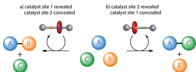
Fig. 1 Different products from a mixture of building blocks using a rotaxane catalyst switchable between two different active sites (e.g. 1/H^+ \cdot CF_3CO_2^- , Fig. 2). Alternative reactions are promoted (involving particular functional groups on different building blocks) according to which active site of the catalyst is revealed (e.g. Fig. 4).
