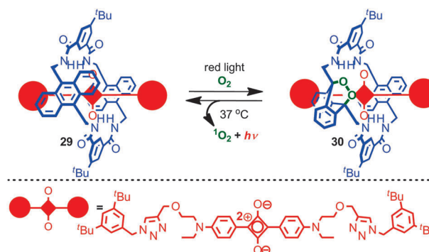
Fig. 17 Smith's NIR chemoluminescent rotaxane. Irradiation of rotaxane 29 with red light leads to formation of endoperoxide 30 which can be stored at -20^\circ\text{C} . 30 undergoes cycloreversion at 37^\circ\text{C} to produce ^1O_2 and regenerate rotaxane 29 .
