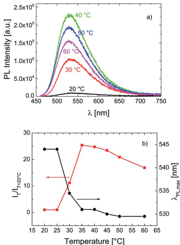
Fig. 2 (a) The evolution of the fluorescence spectrum of P-1 in PBS ( 0.1 \text{ g L}^{-1} ) with temperature, recorded at an excitation wavelength of 450 nm. (b) The correlation between \lambda_{\text{max}}^{\text{PL}} , the relative emission intensity ( I_T/I_{T=20^\circ\text{C}} ), and the temperature of the solution. Data are taken from the spectra in (a).
