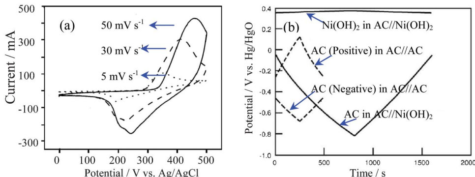
Fig. 15 (a) CV curve of \text{Ni}(\text{OH})_2 in alkaline solution and (b) charge/discharge curves of the positive and negative electrodes in the AC// \text{Ni}(\text{OH})_2 ASC and electric double layer capacitors of AC//AC at 1 \text{ mA cm}^{-2} in 10 \text{ mol l}^{-1} KOH aqueous solution (modified from ref. 87b and 90c).
