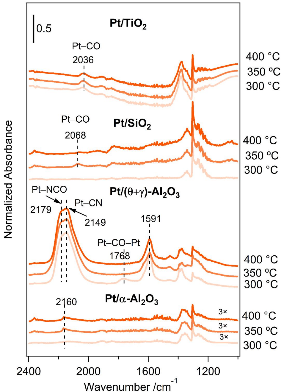
Figure 9. In situ FT-IR spectra for the reaction of CH 4 and NO on the Pt/TiO 2 , Pt/SiO 2 , Pt/( \theta+\gamma )-Al 2 O 3 , and Pt/ \alpha -Al 2 O 3 catalysts at various temperatures.
