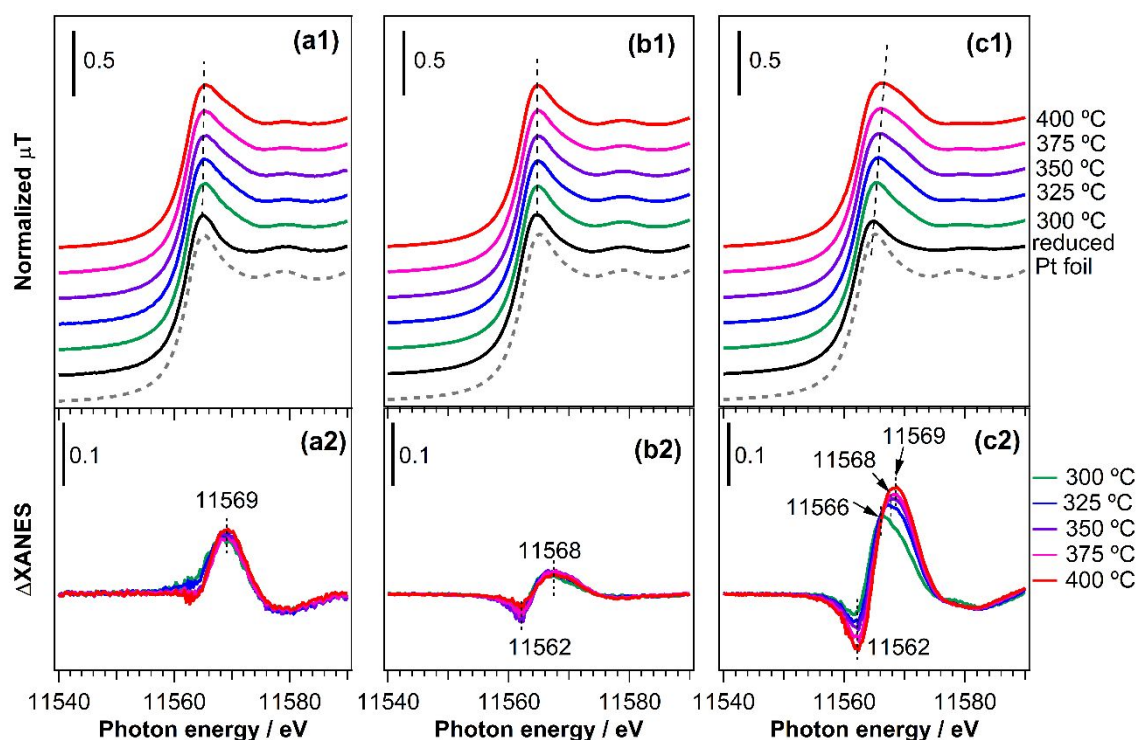
Figure 10. (a1-c1) In situ Pt L 3 -edge XANES spectra for Pt catalysts supported on (a) TiO 2 , (b) SiO 2 , and (c) (θ+γ)-Al 2 O 3 after reduction in H 2 and under the 13.4%CH 4 /1.8%NO/84.8%He reaction mixture at various reaction temperatures. (a2-c2) Difference XANES spectra obtained by subtracting the Pt L 3 -edge XANES spectra of the reduced catalysts from the spectra at the various temperatures.
