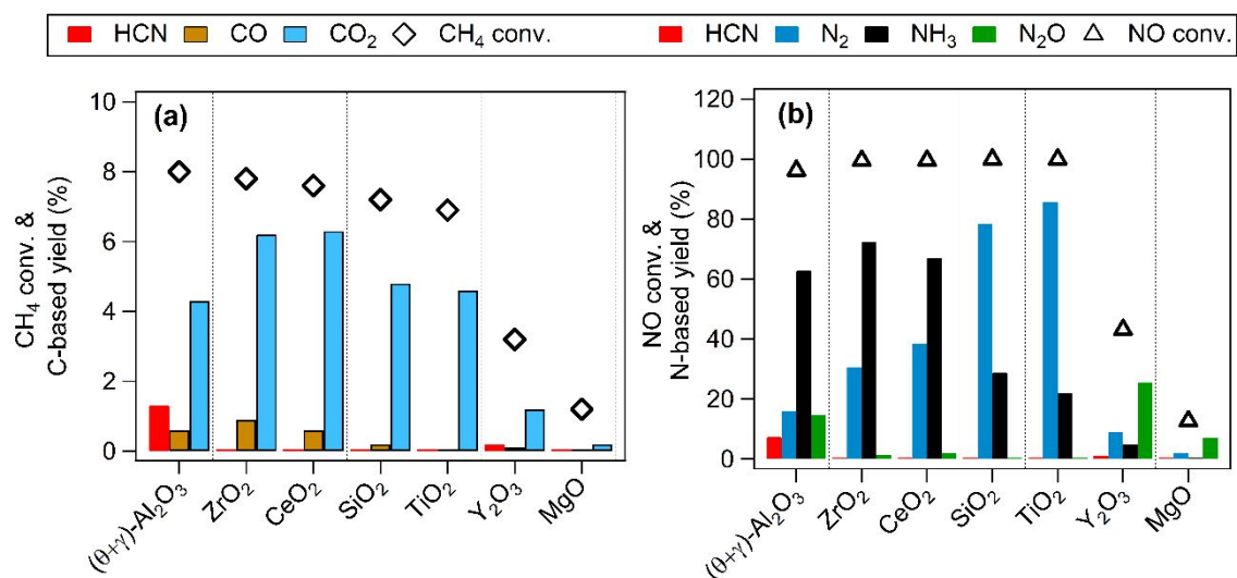
Figure 1. CH 4 oxidation over Pt catalysts supported on different metal oxides. (a) CH 4 conversion and carbon-based product yields and (b) NO conversion and nitrogen-based product yields. Reaction conditions: Catalyst (100 mg), CH 4 /NO/He = 13.4:1.8:84.8, 400 °C, 0.1 MPa, GHSV = 6000 h -1 .
