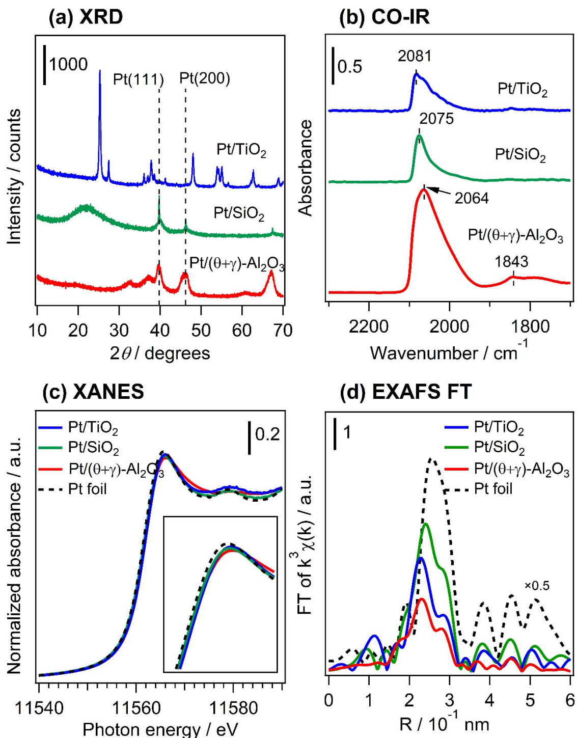
Figure 4. Characterization of the reduced catalysts. (a) XRD patterns, (b) in situ FT-IR spectra of adsorbed CO at 50 °C under He flow, in situ (c) XANES spectra at the Pt L 3 -edge, and (d) Fourier transforms of the Pt L 3 -edge EXAFS ( k^3\chi(k) ) spectra. The samples were reduced at 400 °C in H 2 for 1 h.
