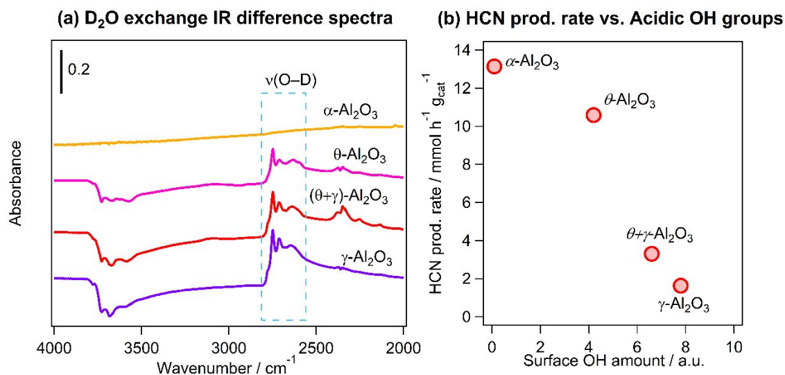
Figure 8. (a) Difference FT-IR spectra of deuterated Pt catalysts supported on Al 2 O 3 with different crystal structures and (b) HCN production rate from the CH 4 –NO reaction at 400 °C vs. amount of surface OH groups determined from (a). Condition for D 2 O exchange: 400 °C for 30 min, evacuation for 15 min (3 times); Reaction conditions: Catalyst (100 mg), CH 4 /NO/He = 13.4:1.8:84.8, 400 °C, 0.1 MPa, GHSV = 6000 h -1 .
