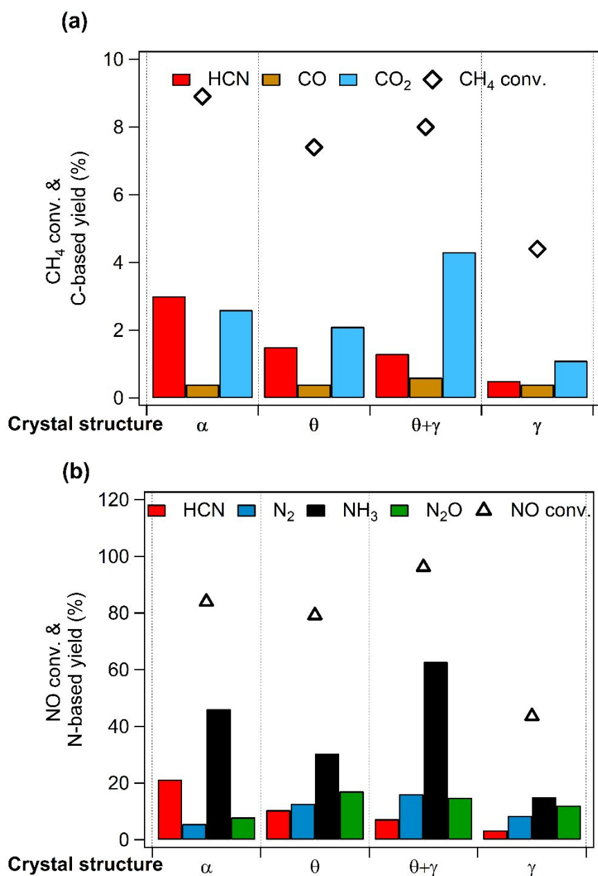
Figure 6. CH 4 oxidation over Pt catalysts supported on Al 2 O 3 with different structures. (a) CH 4 conversion and carbon-based product yields and (b) NO conversion and nitrogen-based product yields. Reaction conditions: Catalyst (100 mg), CH 4 /NO/He = 13.4:1.8:84.8, 400 °C, 0.1 MPa, GHSV = 6000 h -1 .
