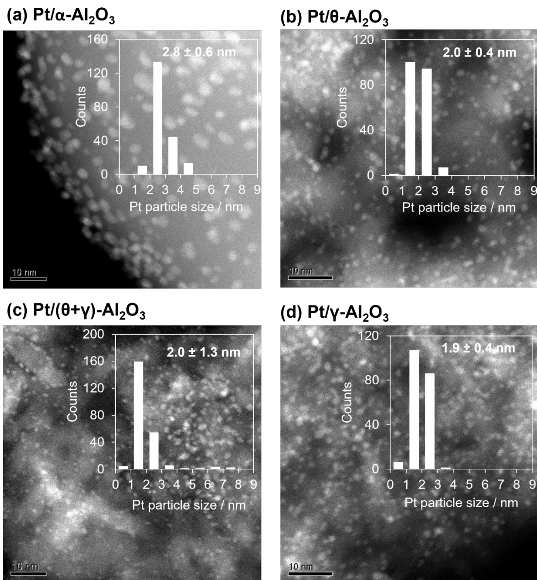
Figure 5. STEM images and particle size distributions of Pt nanoparticles supported on Al 2 O 3 with different crystal structures. The size distributions were measured from >200 particles and were used to determine mean surface particle diameters (shown along with standard deviations).
