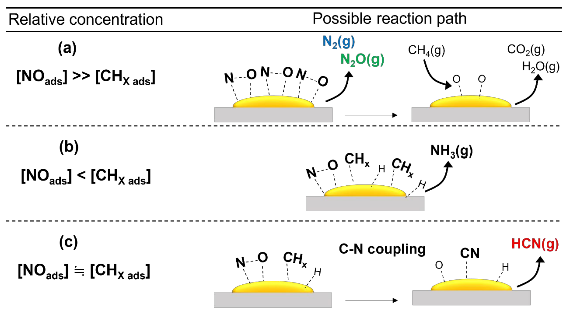
Scheme 1. Schematic depiction of effects of relative concentration of adsorbed species on the products formed from the CH 4 and NO reaction
