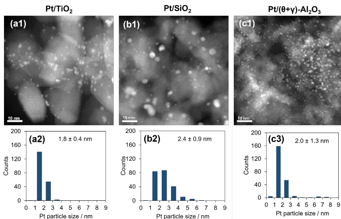
Figure 3. TEM images (a1-c1) and particle size distributions (a2-c2) of Pt catalysts supported on (a) TiO 2 , (b) SiO 2 , and (c) (θ+γ)-Al 2 O 3 . The size distributions were measured from >200 particles and were used to determine mean number particle diameters (shown along with standard deviations).
